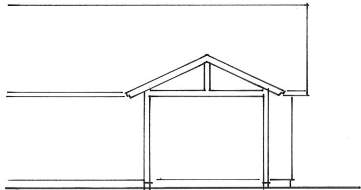
FASAD FRONT
