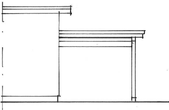
FASAD FRONT
